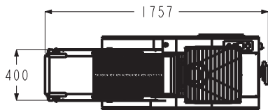
AUTOMATIC DIVIDER WITHOUT PRE-ROUNDER HOPPER 40L
