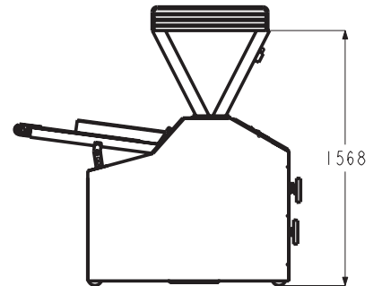
HOPPER 120L
