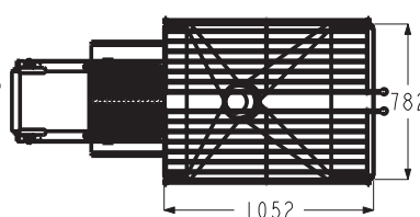
HOPPER 200L
