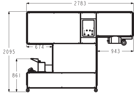
INTERMEDIATE PROOFER 93A 276 USEFUL PIECES
