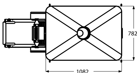
HOPPER 200L
